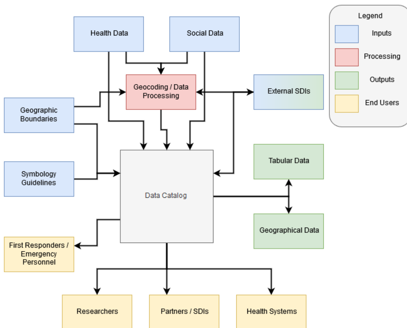
Figure 7. Generalized Health SDI Architecture.
