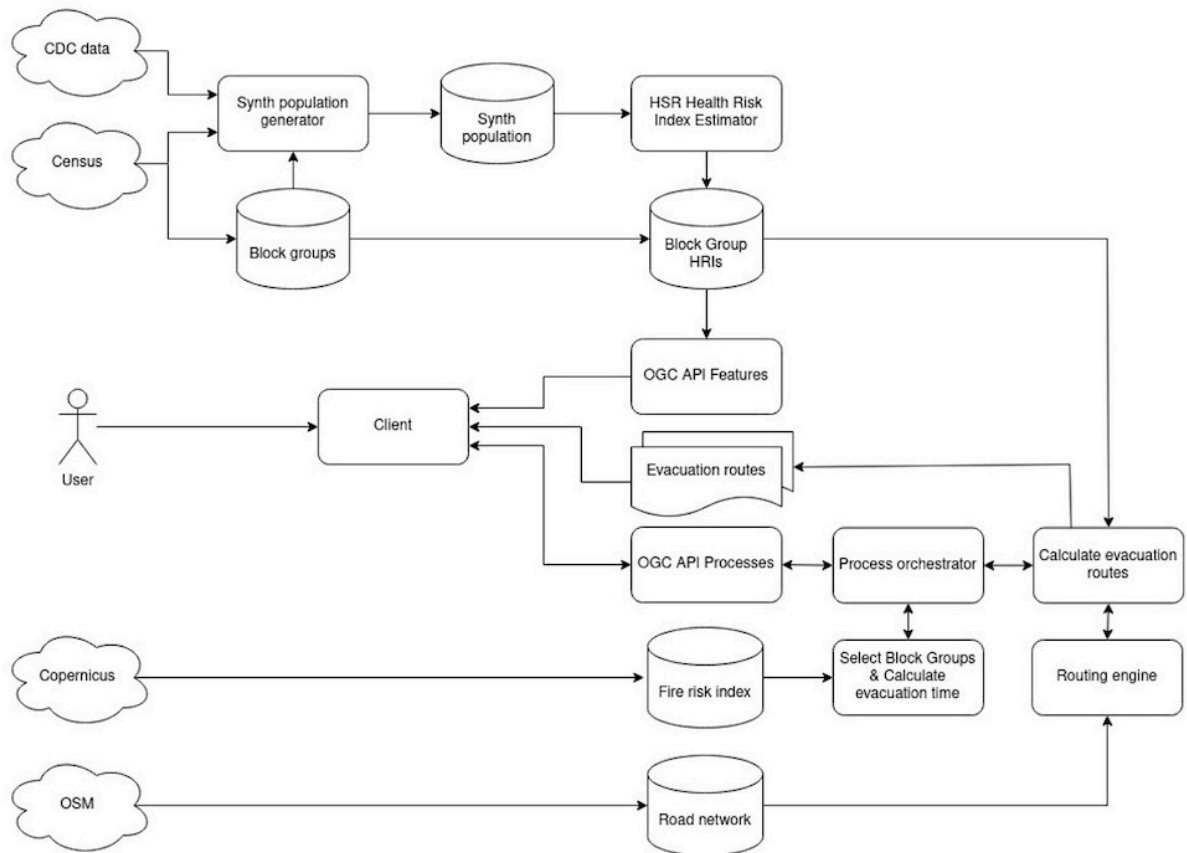
Figure 5 – D109 Technical implementation schema
