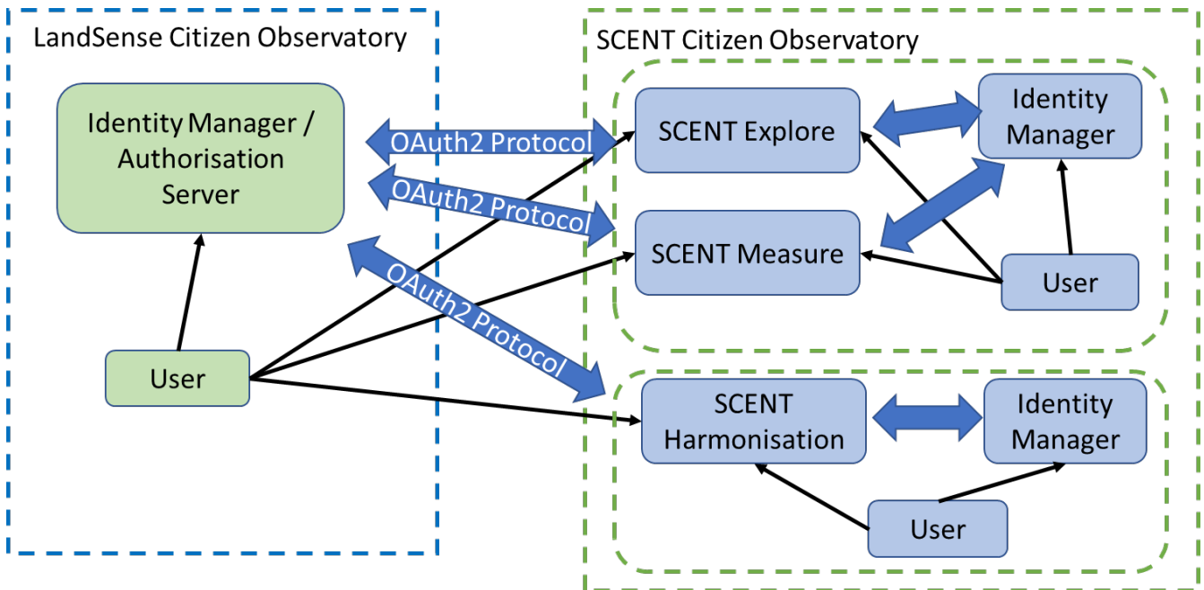
Figure 54. Architectural overview of integration between SCENT applications and LandSense authorisation server
