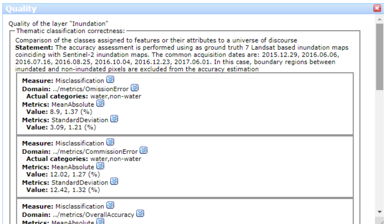
Figure 16. Data Quality indicators presented following the QualityML data model.
