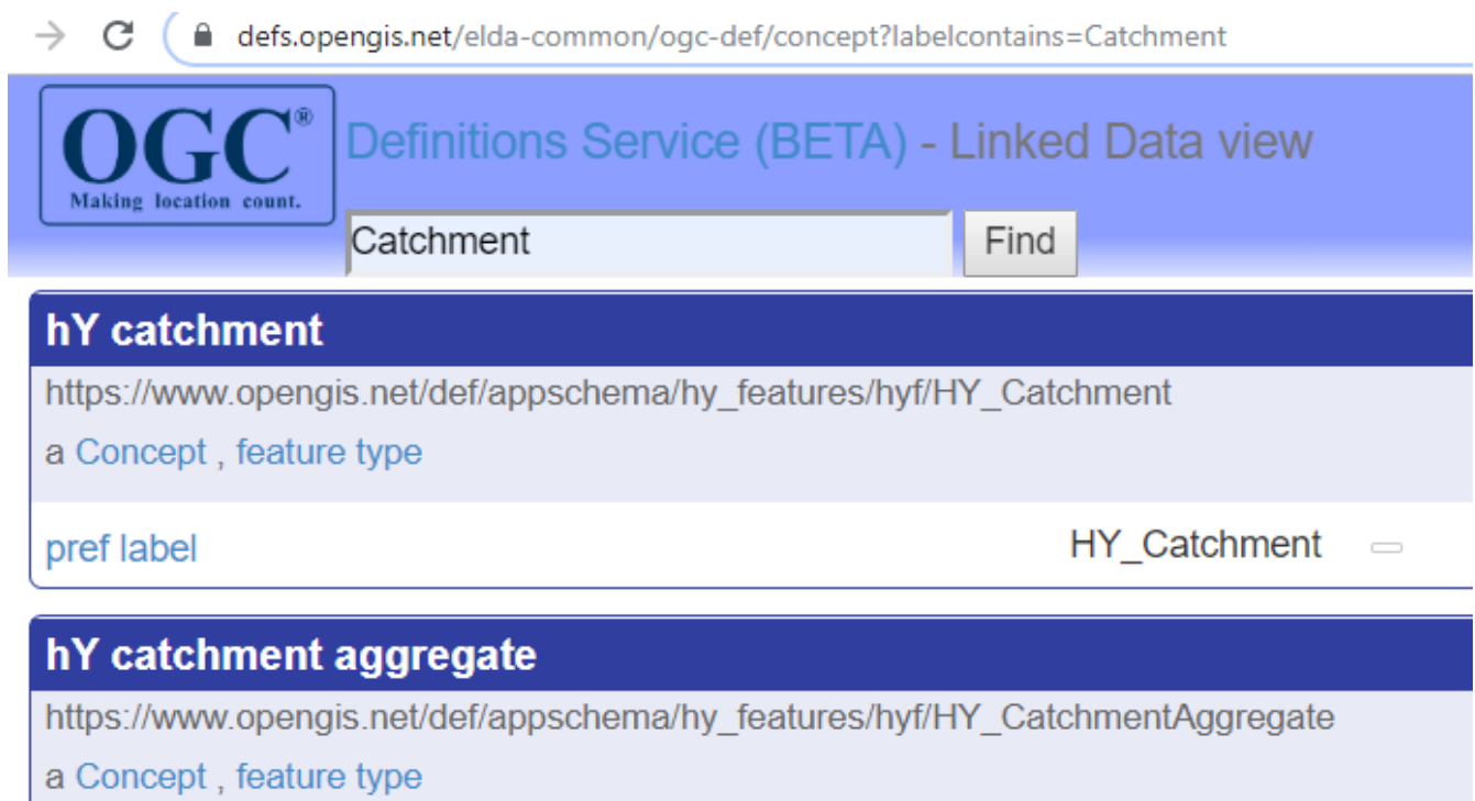
Figure 39. Search option
