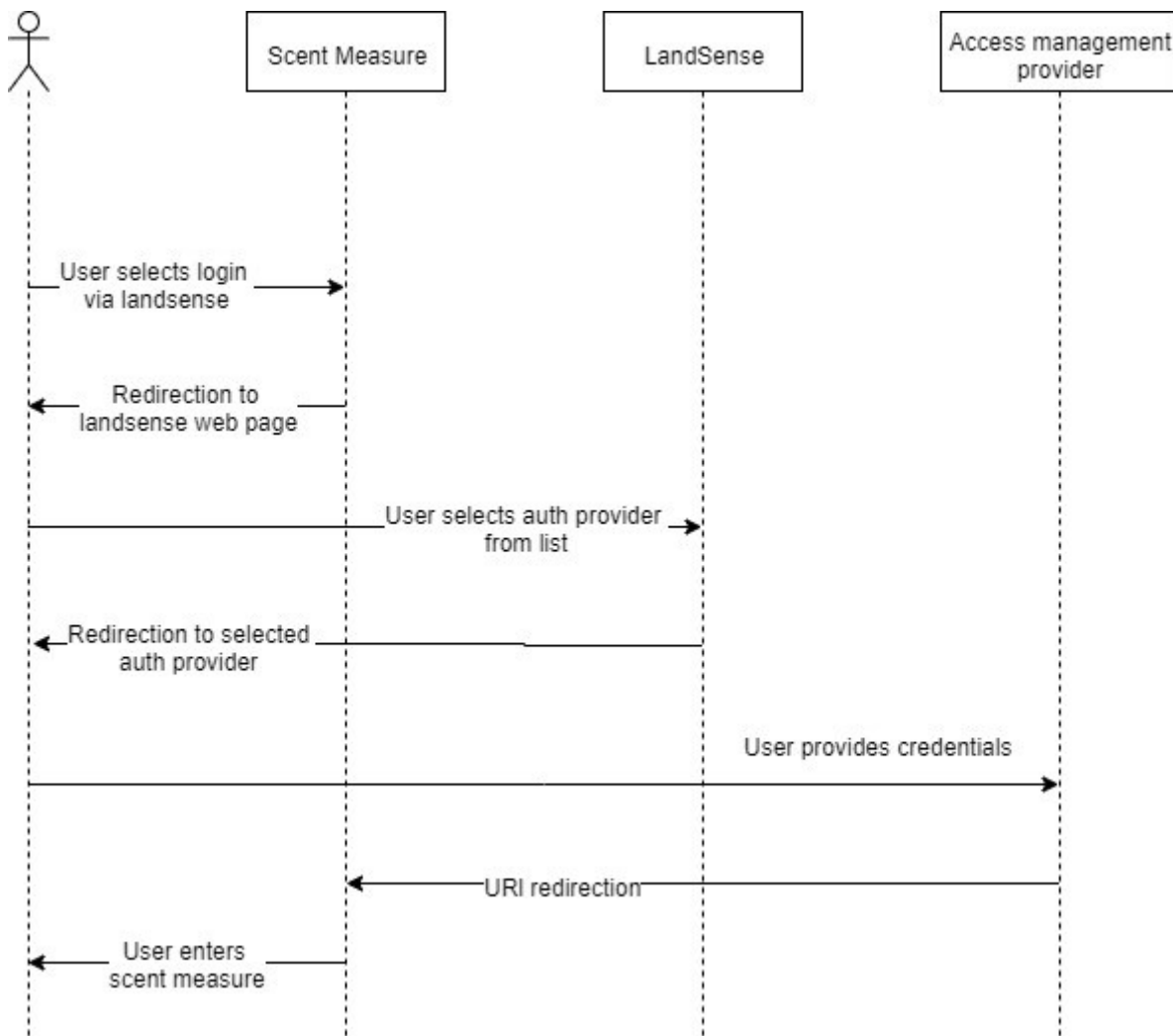
Figure 56. Login sequence diagram for Scent Measure
