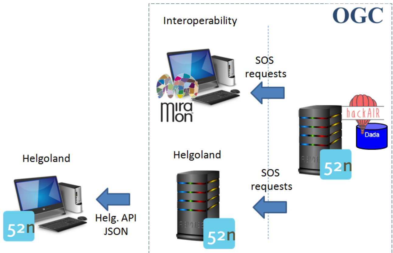
Figure 8. Helgoland SOS Architecture
