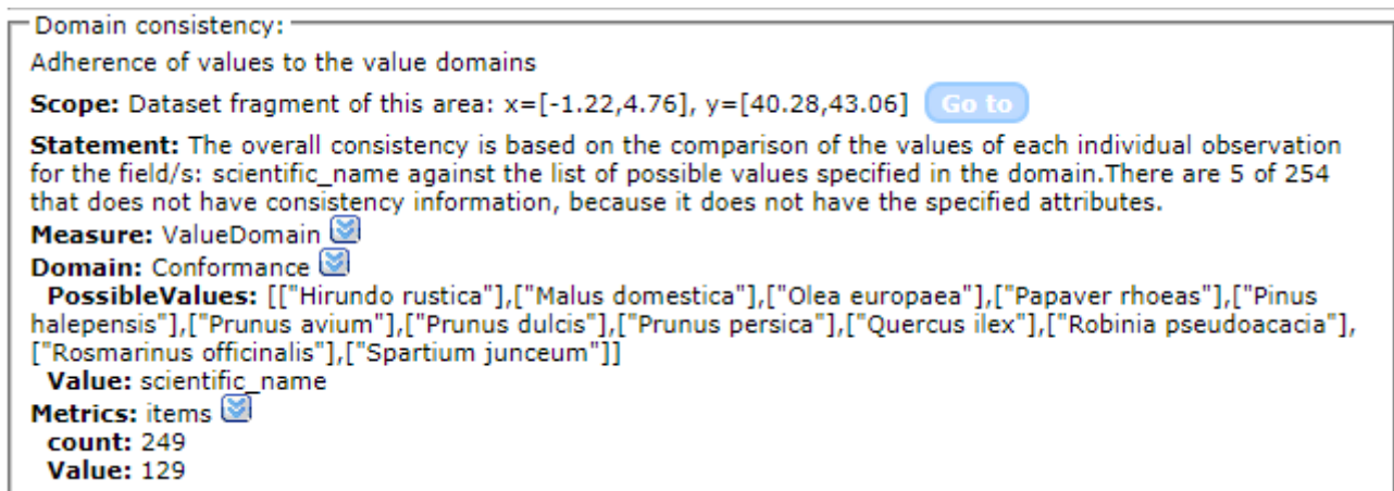
Figure 24. Domain consistency result
