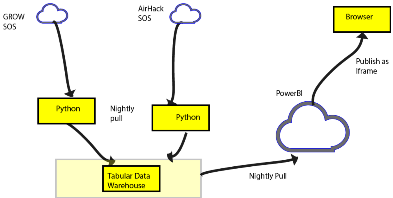
Figure 10. GROW data follow
