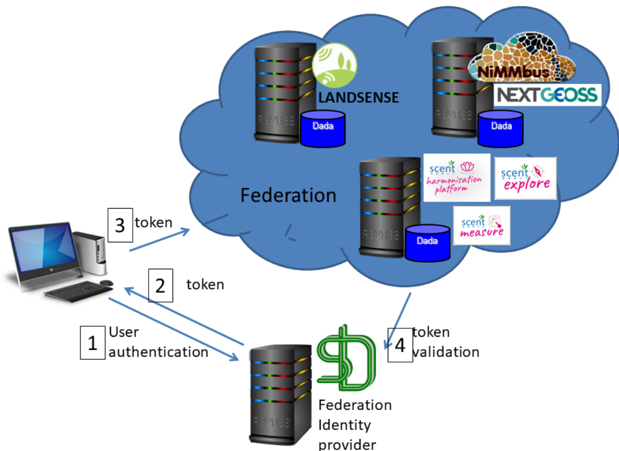
Figure 42. Federation diagram
