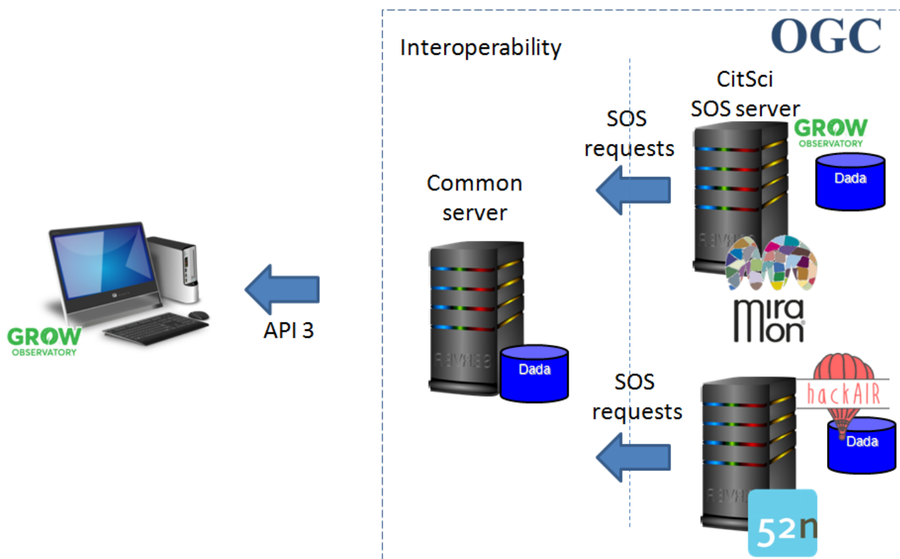
Figure 6. Grow SOS Architecture
