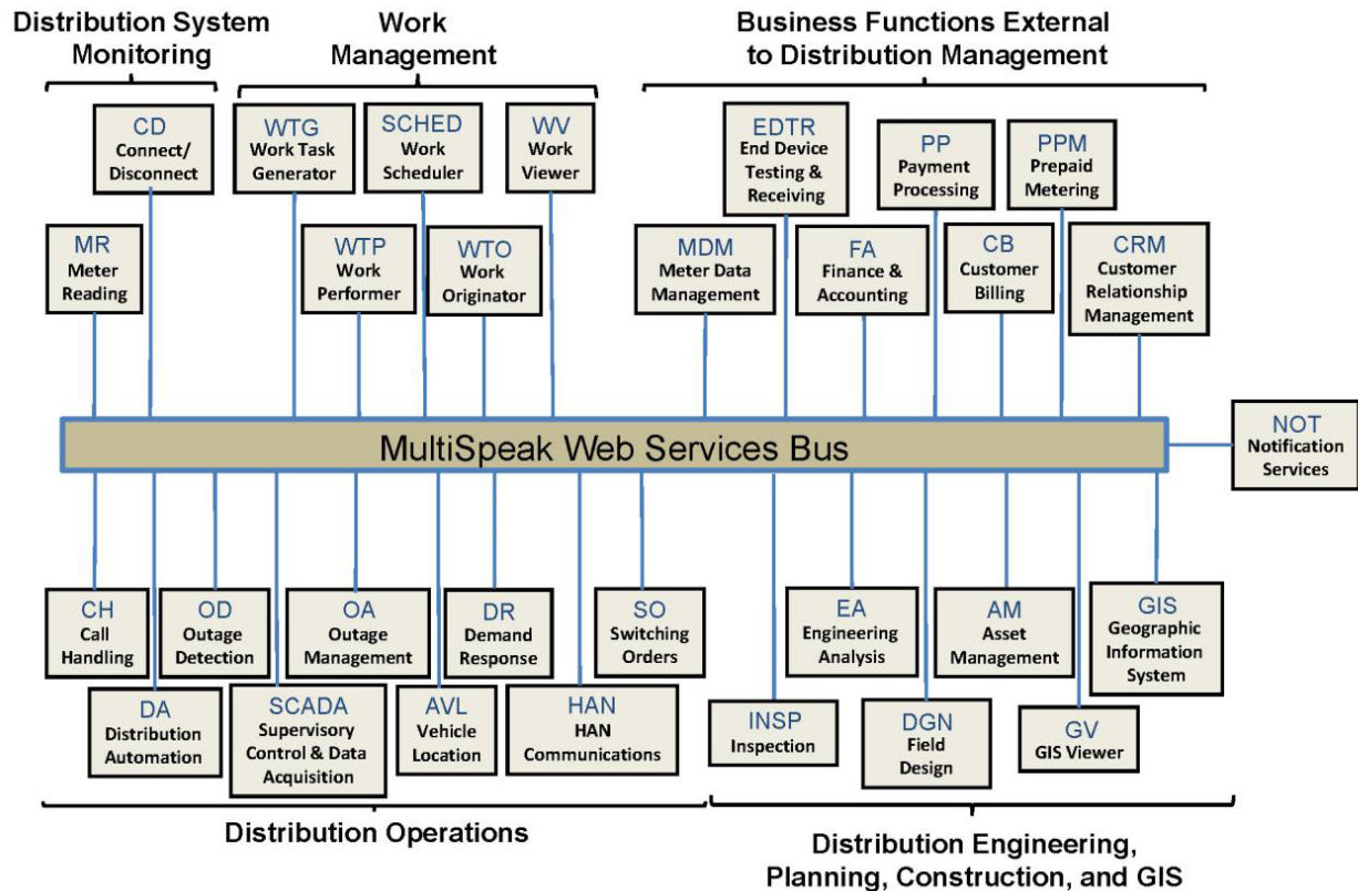
Figure 6. MultiSpeak Process Model Overview
