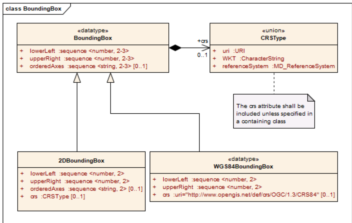
Figure 3 — BoundingBox UML model
