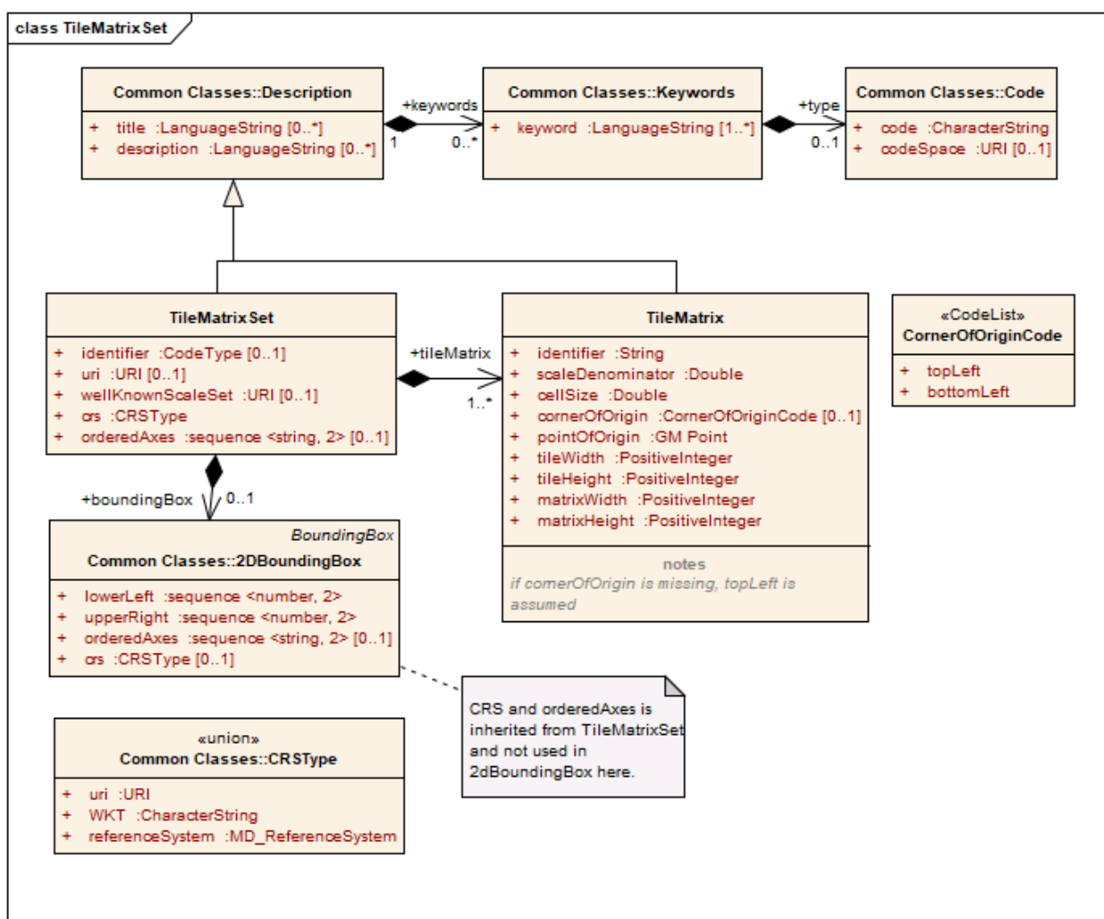
Figure 9 – TileMatrixSet UML model
