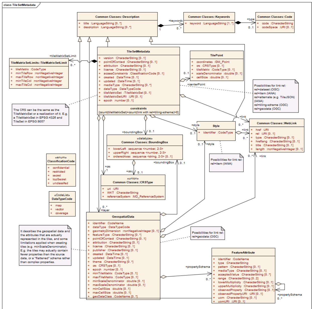
Figure 13 – TileSetMetadata UML model
