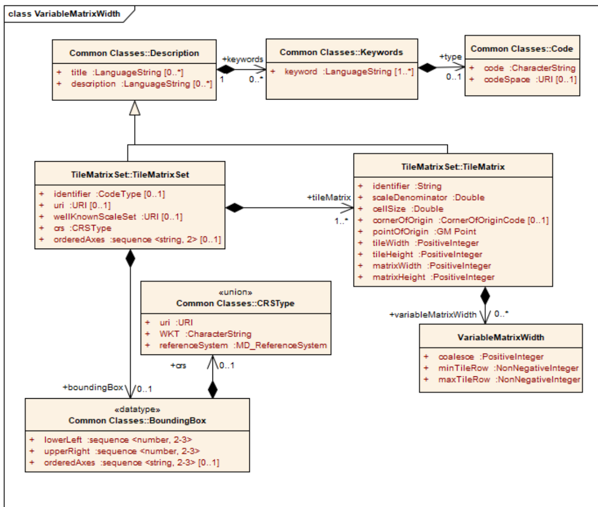
Figure 10 – VariableMatrixWidth UML model
