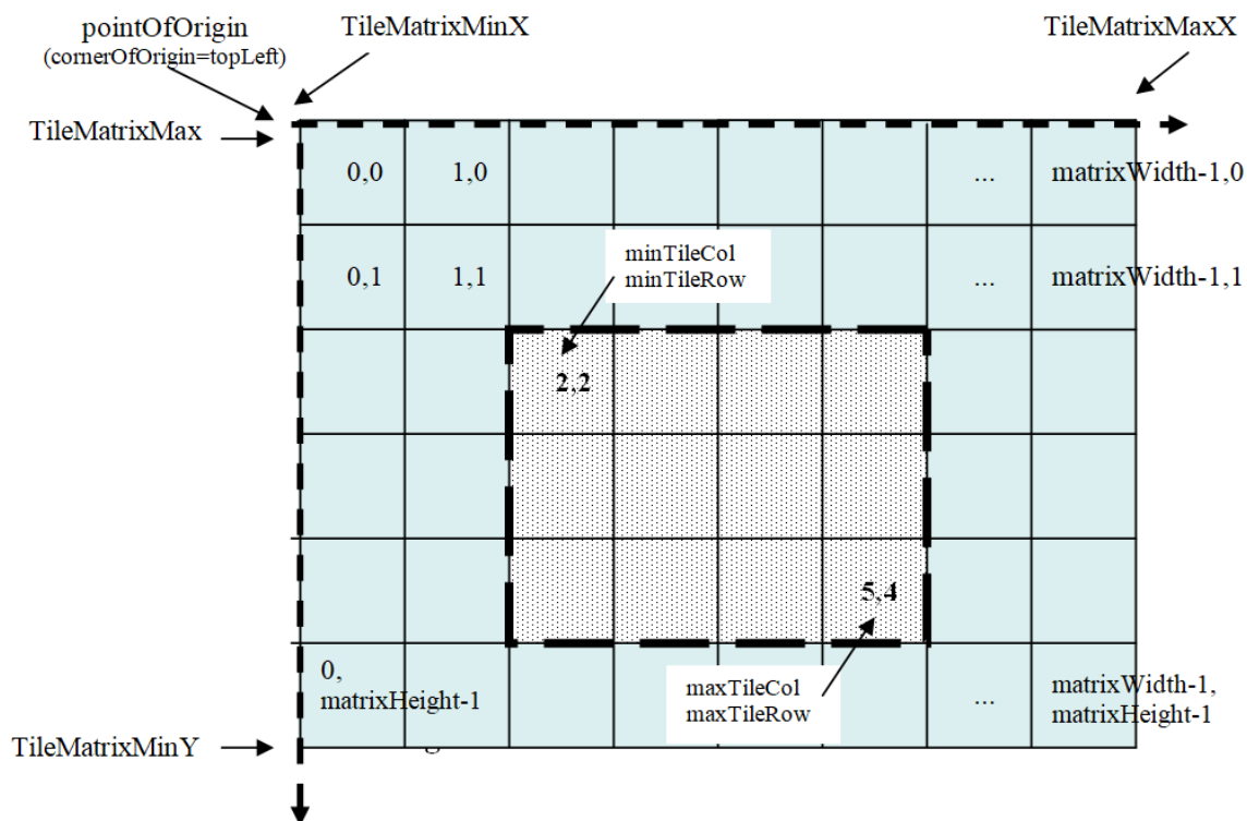
Figure 11 – TileMatrixSet Limits
