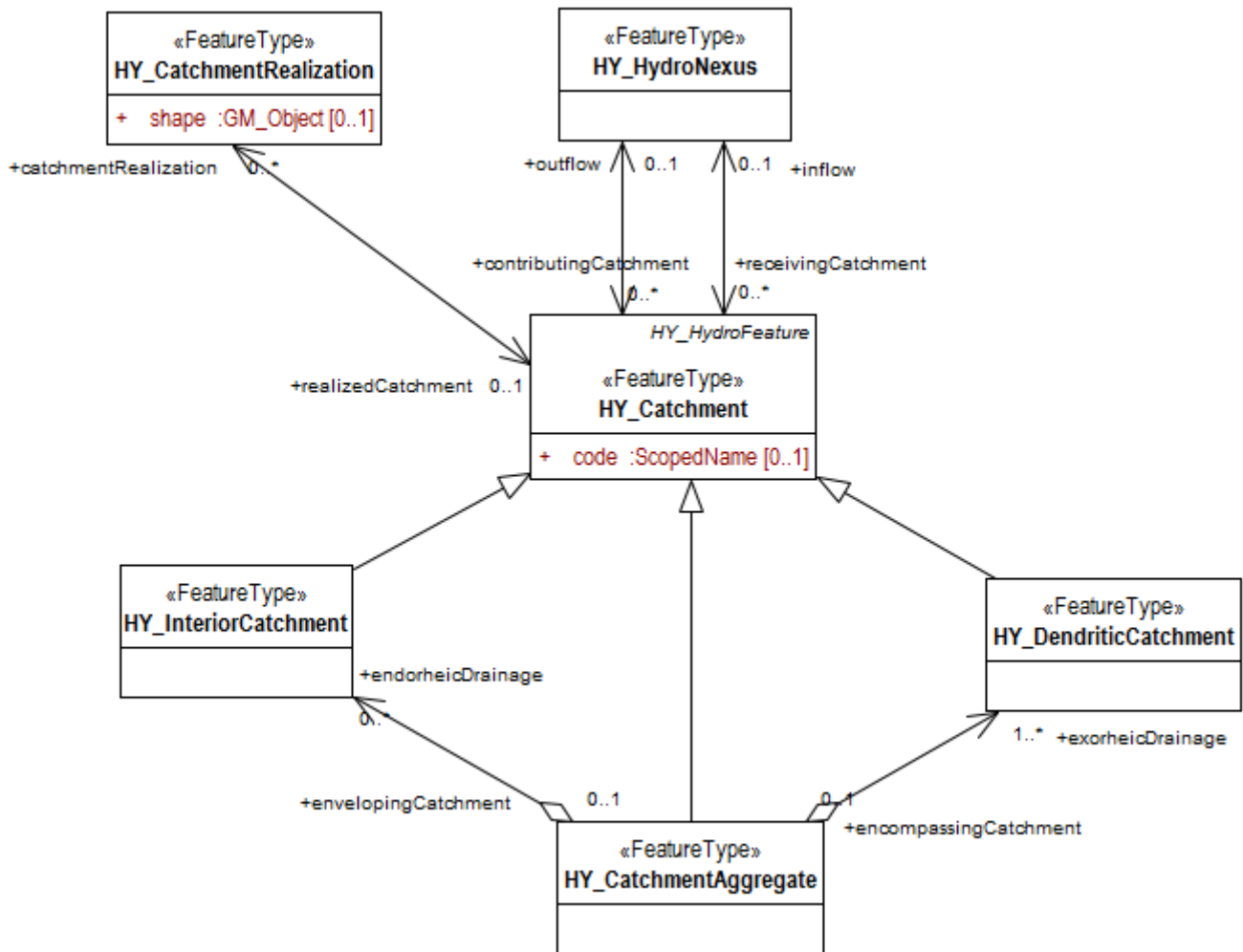
Figure 25. Catchment model (UML class diagram)
