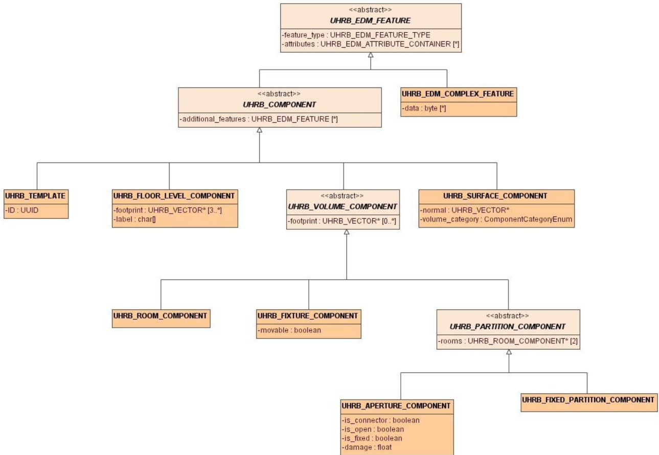
Figure A-4: UHRB Class Diagram
