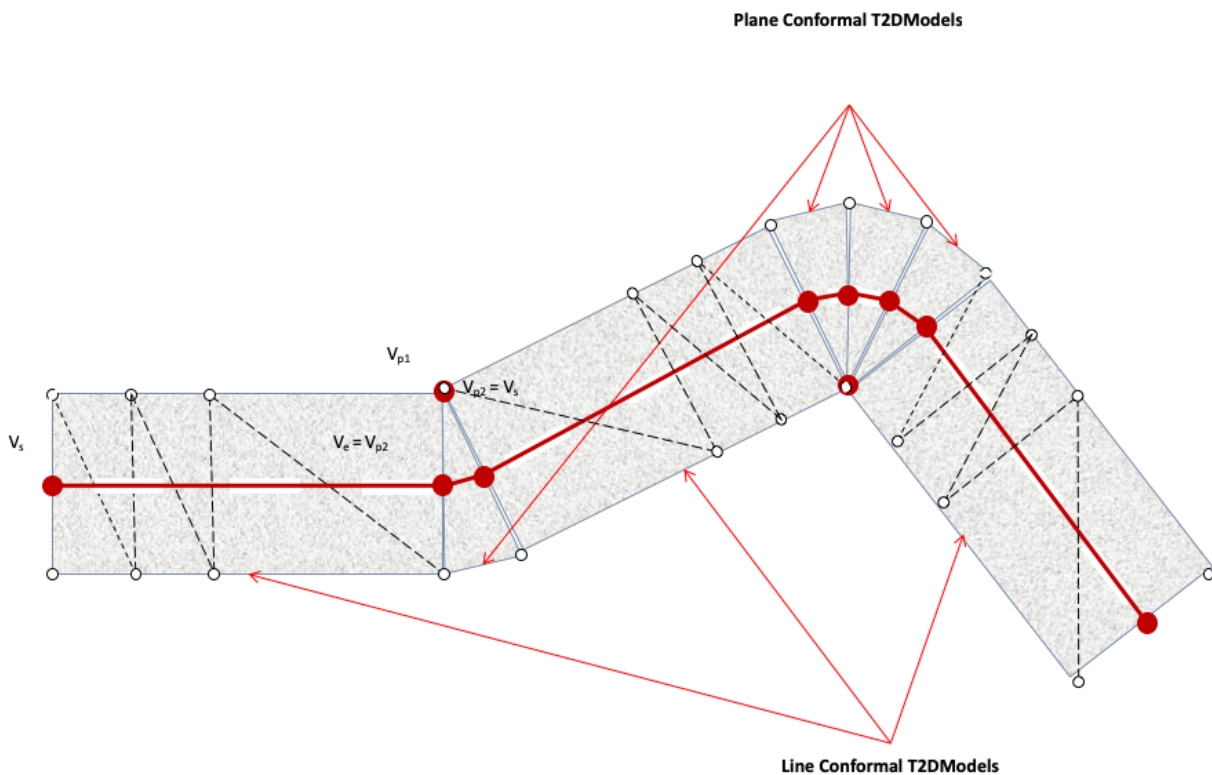
Figure 6-40. Plane Conformal Mode
