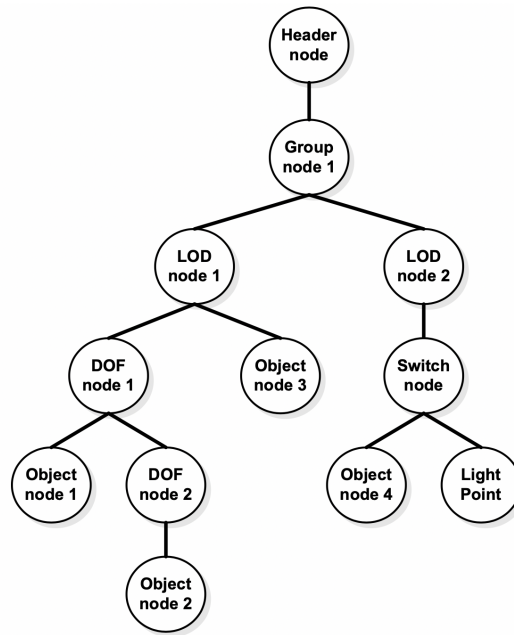
Figure 6-1. General OpenFlight Tree Structure
