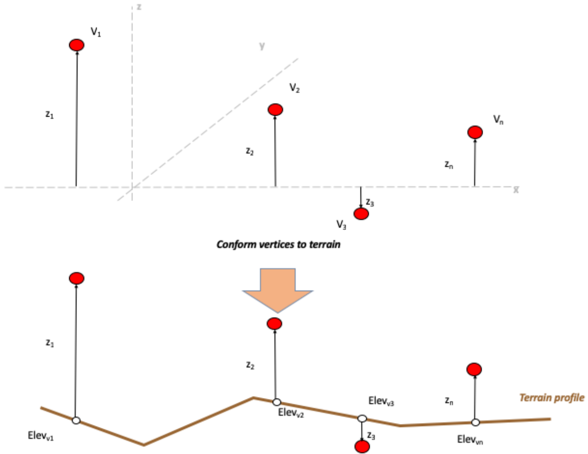
Figure 6-36. Conforming Vertices to Terrain
