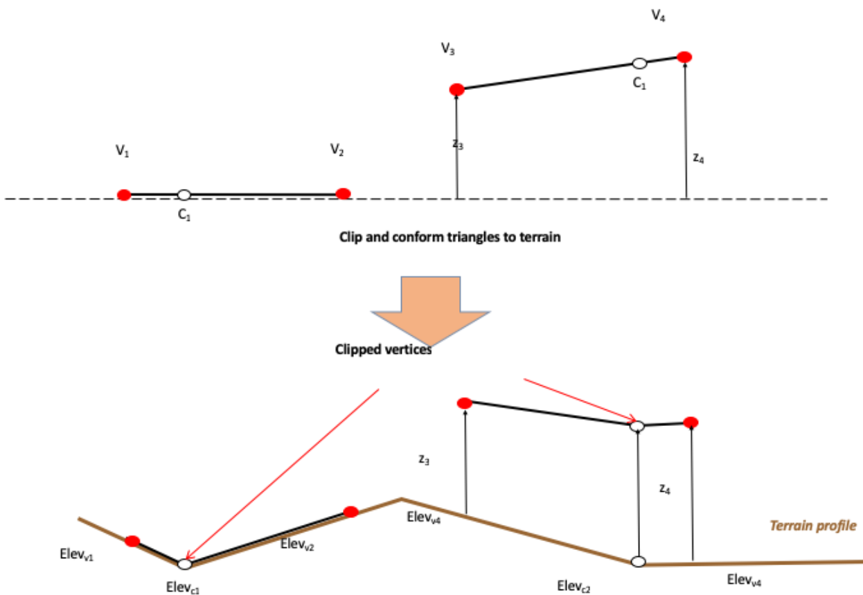
Figure 6-42. Surface Conformal Mode
