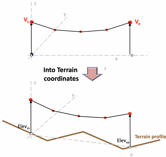
Figure 6-39. Line Conformal Mode
