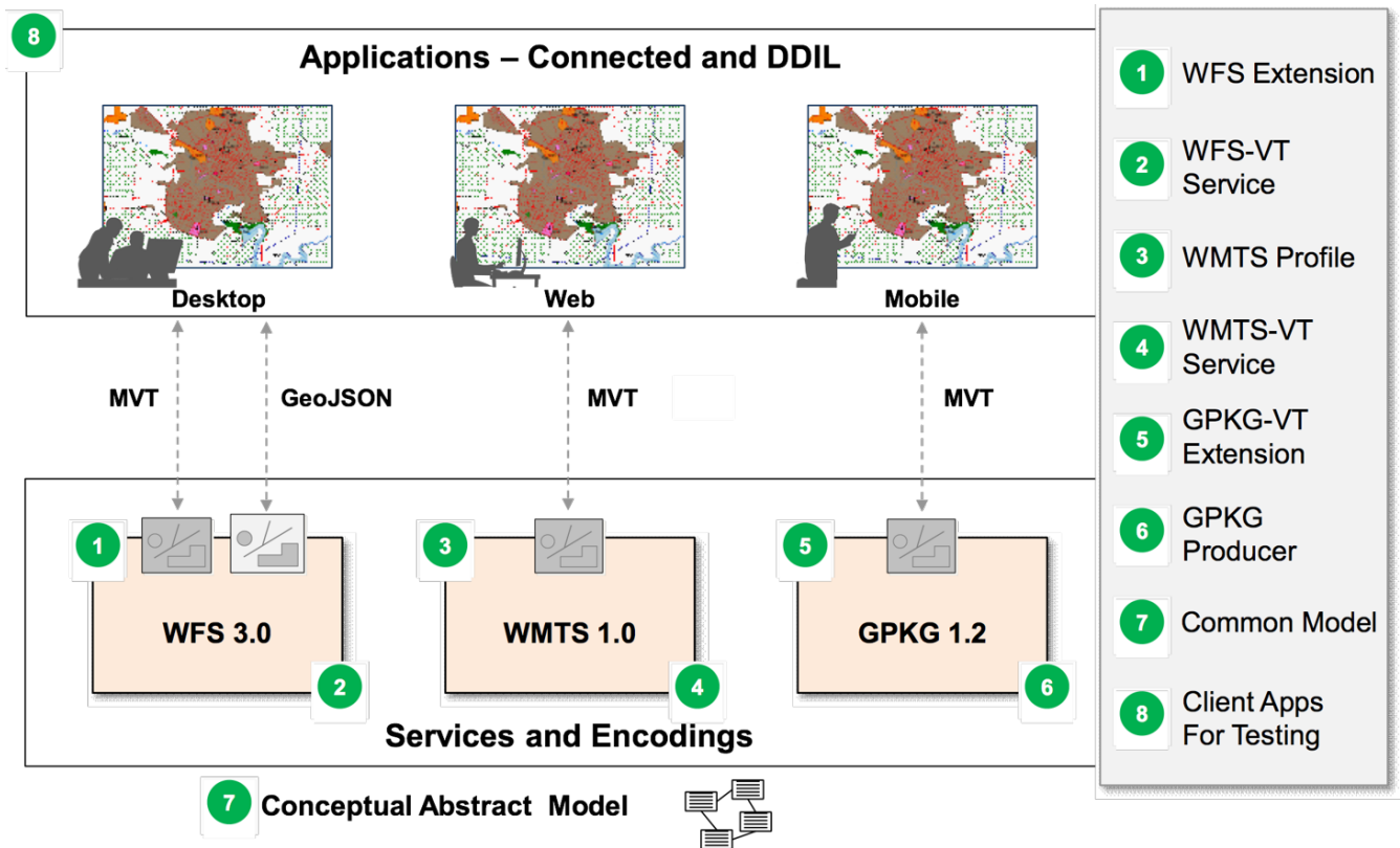
Figure 1. Vector Tiles Pilot Architecture
