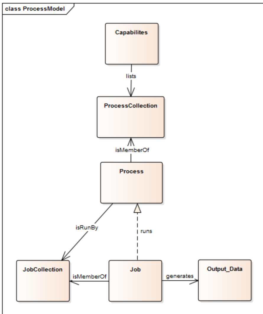
Figure 11. Resource model of the WPS REST server
