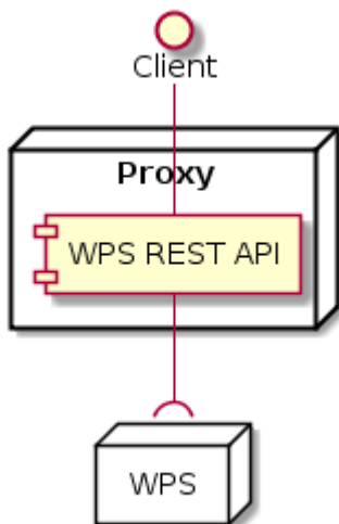
Figure 12. Architecture of the 52°North WPS REST API implementation
