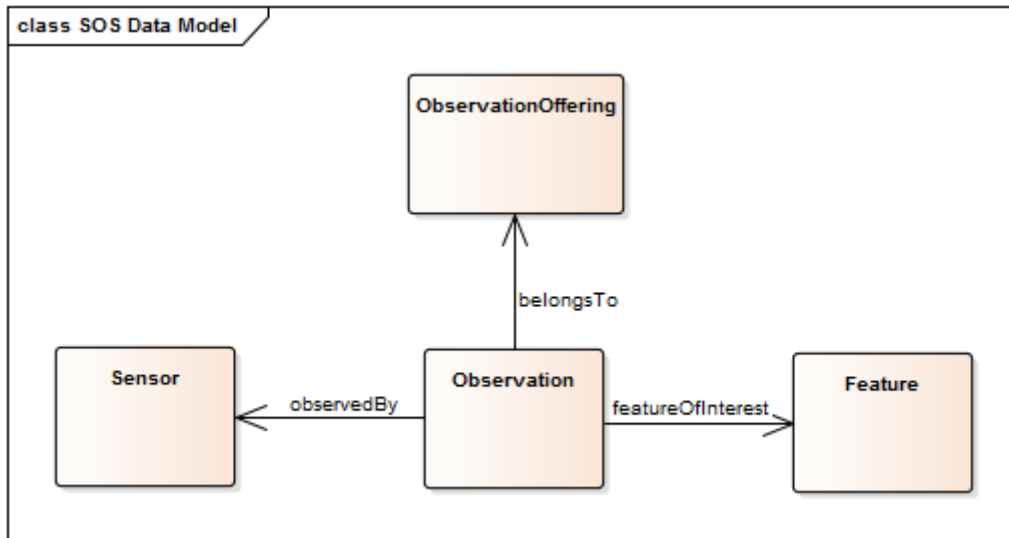
Figure 3. Simplified resource model of the Sensor Observation Service
