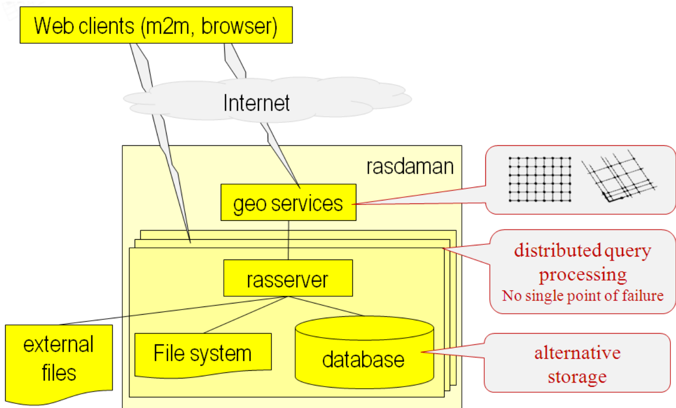
Figure 7. rasdaman Architecture
